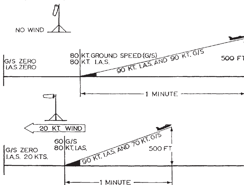
Fig 4-2 Advantages of Taking-Off into Wind
