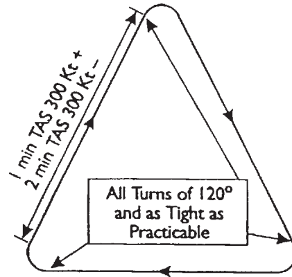
Fig 6-2 Receiver Only Operating
