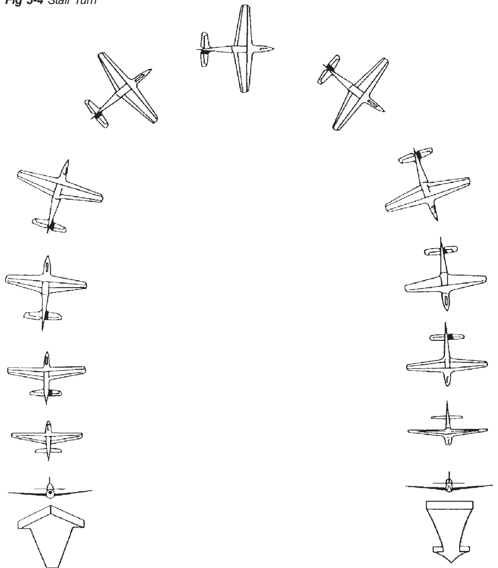
Fig 5-4 Stall Turn
